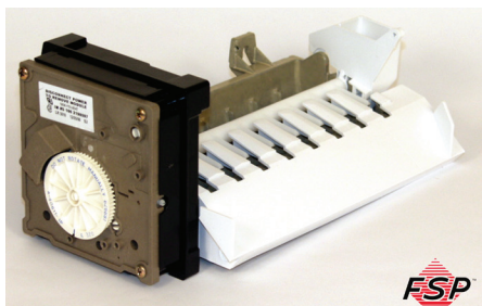
Whirlpool Icemaker 2198597
